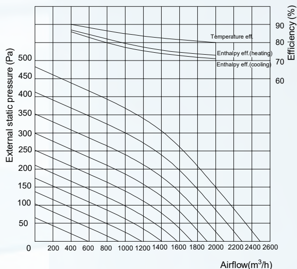
■ CFA 2000C Performance Chart
