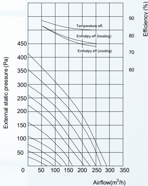
■ CFA 250C Performance Chart
